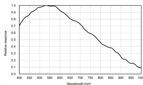
MV-CE200-10UM
